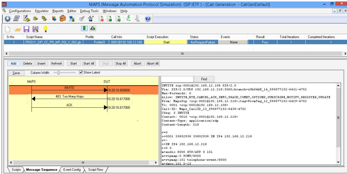
Figure: Proxy Conformance Script
