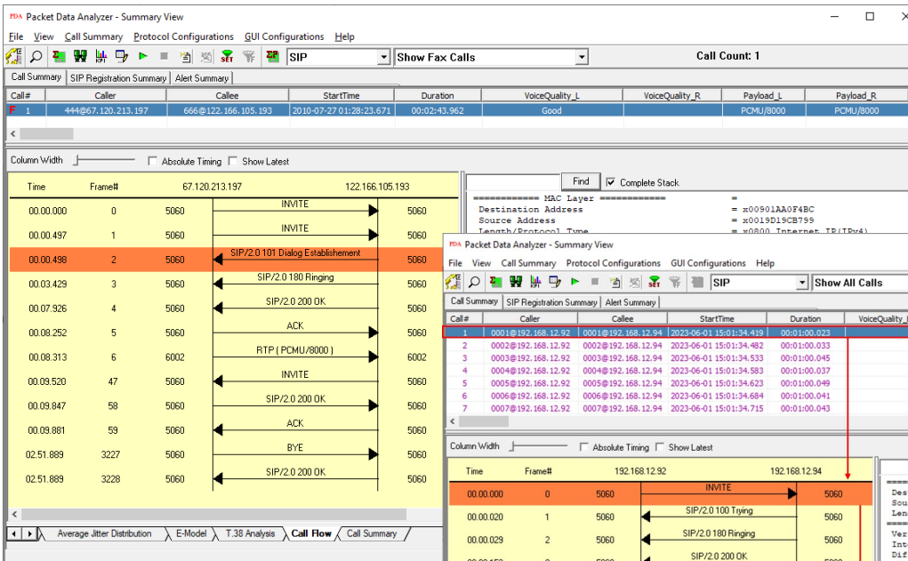
FAX Call Flow
