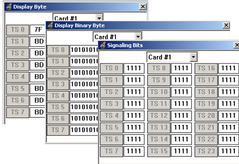
Monitor Byte, Binary Byte, and Signaling Bits
